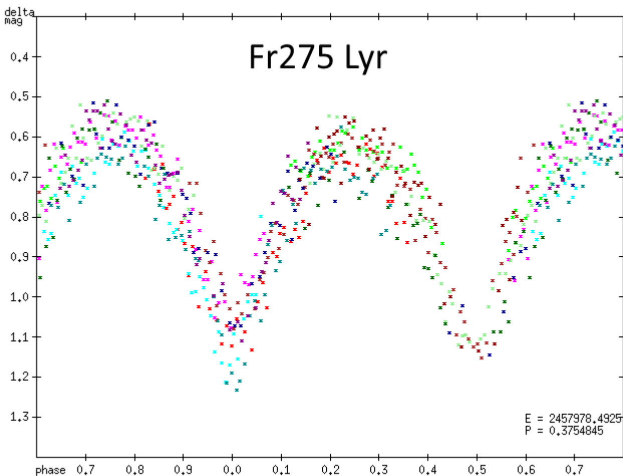
Fig 10: Phased lightcurve of Fr275 Lyr = UCAC4 597-069471 using the ephemeris given above. FLI Proline 16803+V-filter (2016-2017). Presented elements were calculated by taking into account all minima (see tables below) with the method of least squares.
