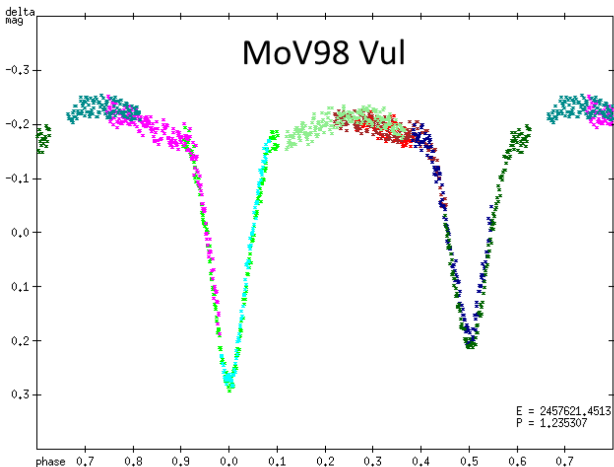
Fig 4: Phased lightcurve of MoV98 Vul = UCAC3 236-212219 using the ephemeris given above. FLI Proline 16803+V-filter (2016-2017). Presented elements were calculated by taking into account all minima (see tables below) with the method of least squares.
